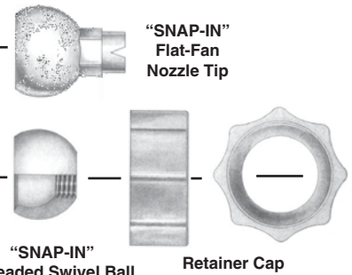
Retainer Cap
